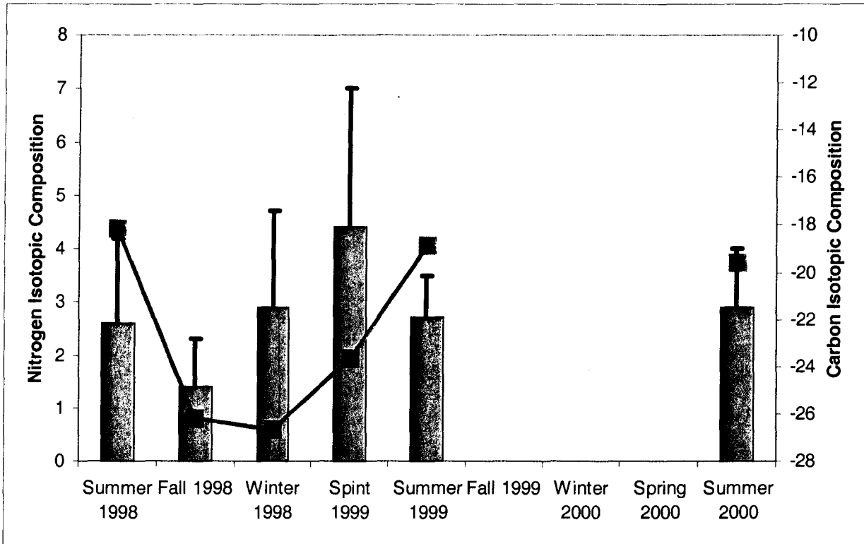
Figure 3: Ranges and means of \delta^{13}\text{C} and \delta^{15}\text{N} values measured on POM from the Florida Keys between 1998 and 2000. Bars = nitrogen, symbols = carbon. Error bars = 1 standard deviation.
