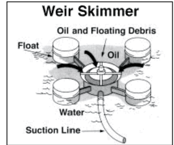
In a weir skimmer, oil floating on the surface of the water is pumped into storage after flowing over the skimmer's weir, which is maintained at the oil/water interface.
