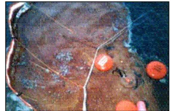
A skimmer from the U.S. Coast Guard's Vessel of Opportunity Skimming System (VOSS) removes oil contained by the system's boom. Photo: USCG
