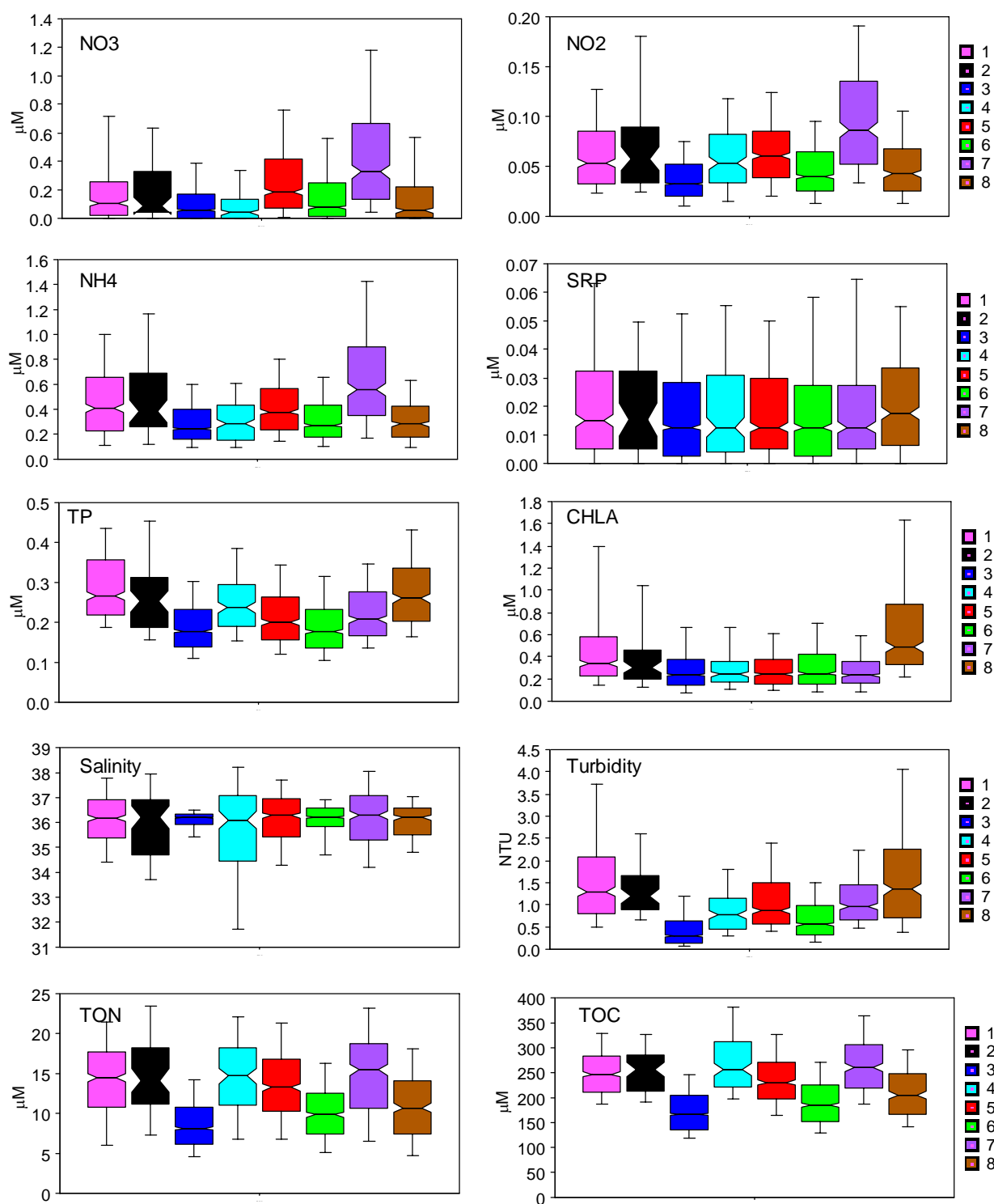
Figure 4. Box-and-whisker plots showing median and distribution of \text{NO}_3^- , \text{NO}_2^- , \text{NH}_4^+ , SRP, TP, CHLA, salinity, turbidity, TP, TON, and TOC stratified by water quality cluster. Notches in the box that do not overlap with another are considered significantly different.
