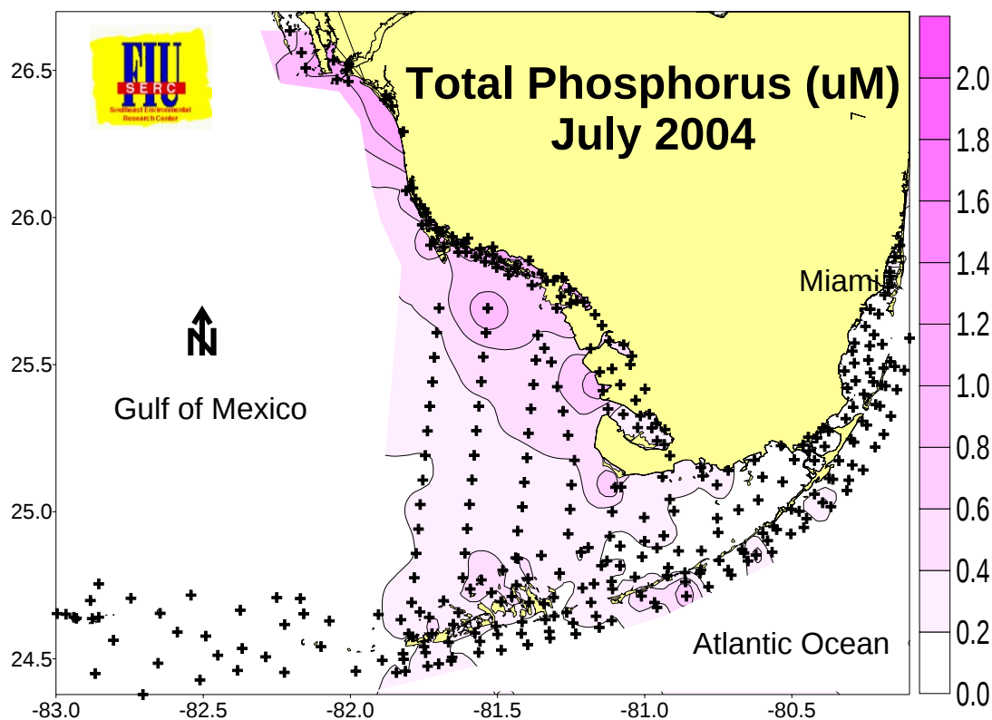
Figure 21. Example of total phosphorus distributions across the region during summer 2004.
