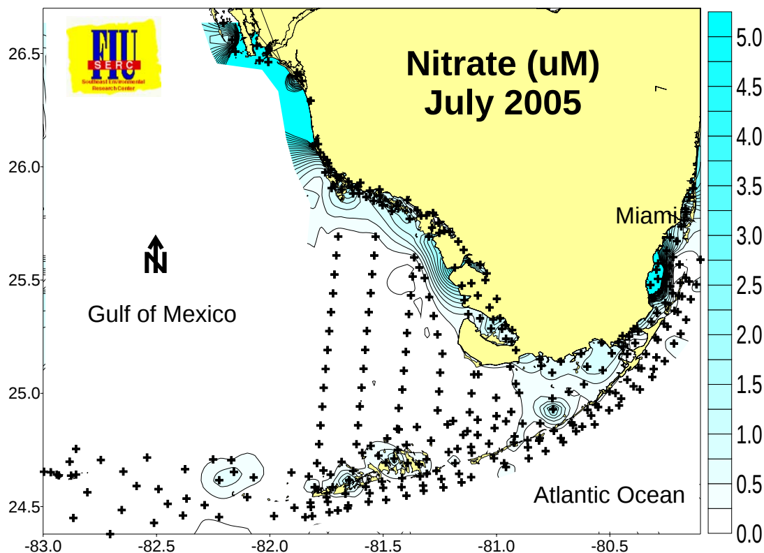
Figure 20. Example of nitrate distributions across the region during summer 2005.
