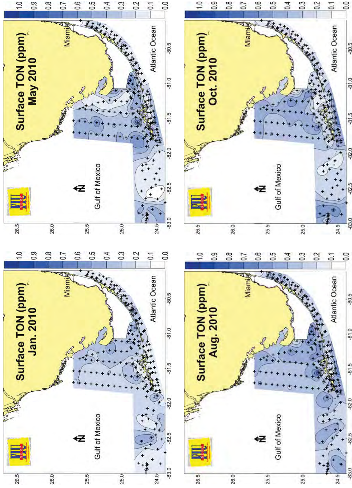
Figure 34. Distributions of surface total organic nitrogen across the region during 2010.
