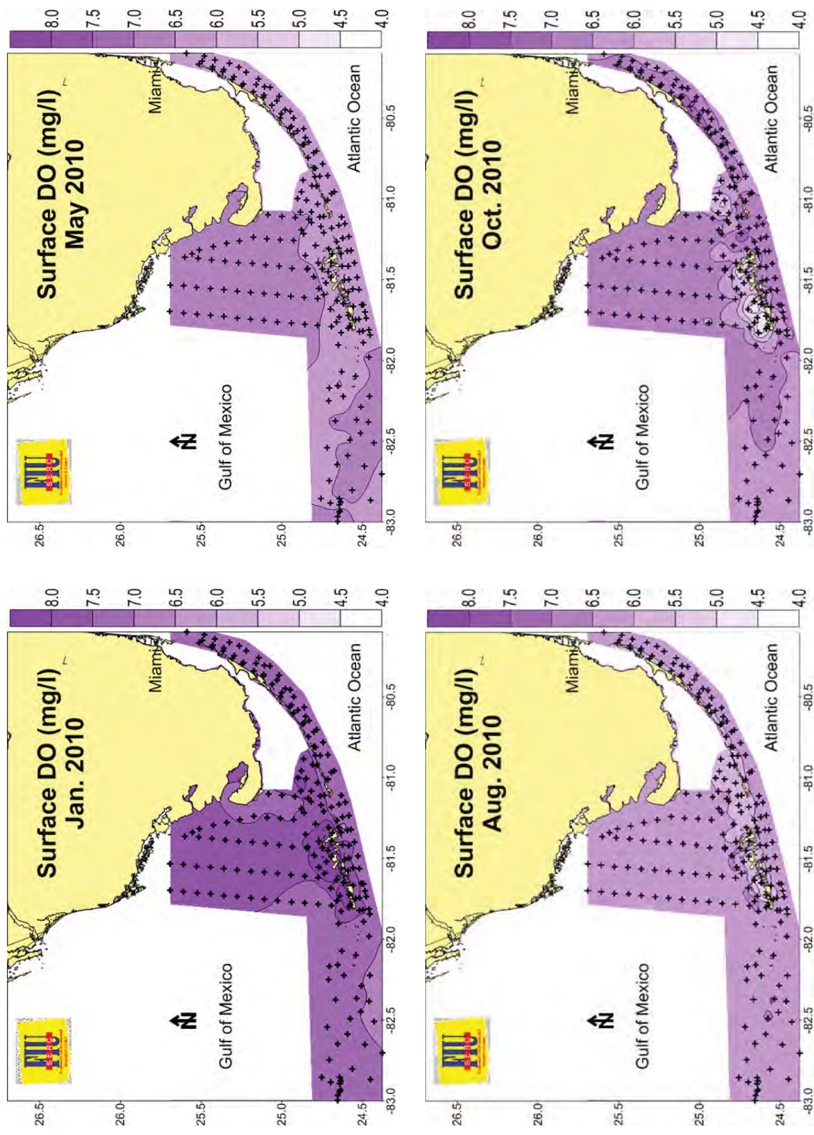
Figure 26. Surface dissolved oxygen distributions across the region during 2010.
